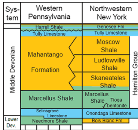
Figure 3. Stratigraphy of the Devonian Shale
